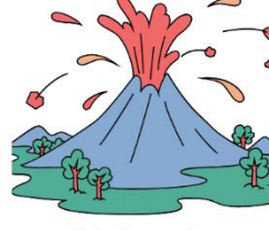
Volcanic Eruption
