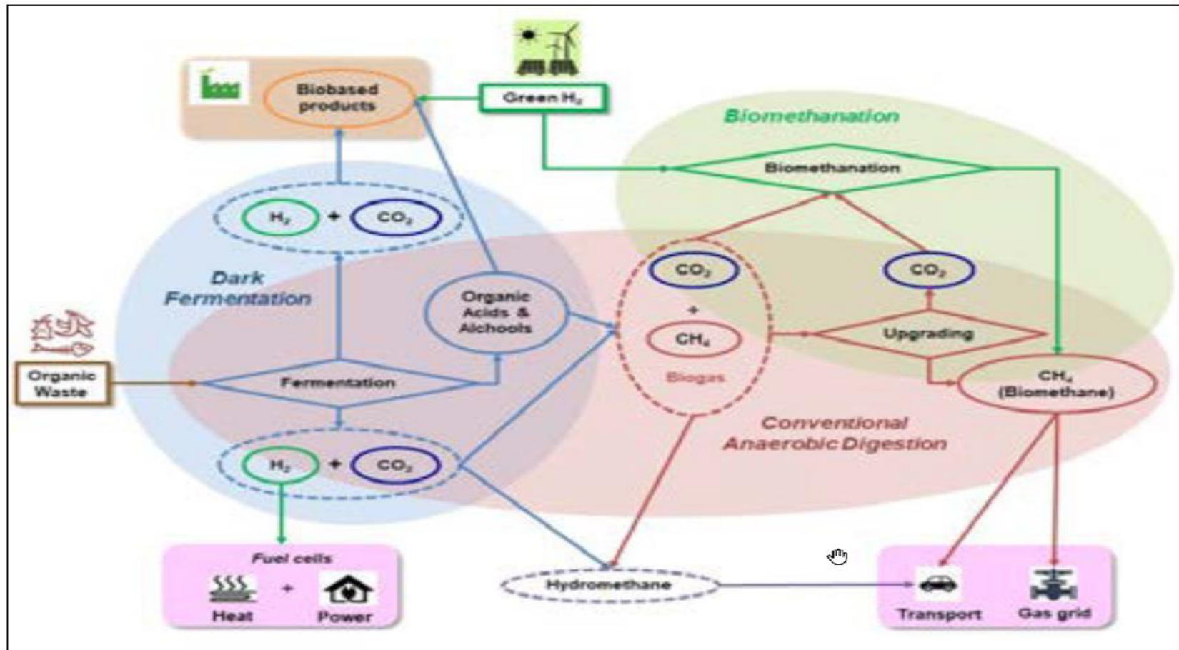
Fig.1 Biological processes integrated in the green H 2 value chain: Background coloured areas enclose the main step of each process; Rectangles represent processes; feeding Diamond shapes represent technological stages; Round shapes represent products; Dotted lines enclose gas mixtures; Background coloured rectangles represent the end uses.
